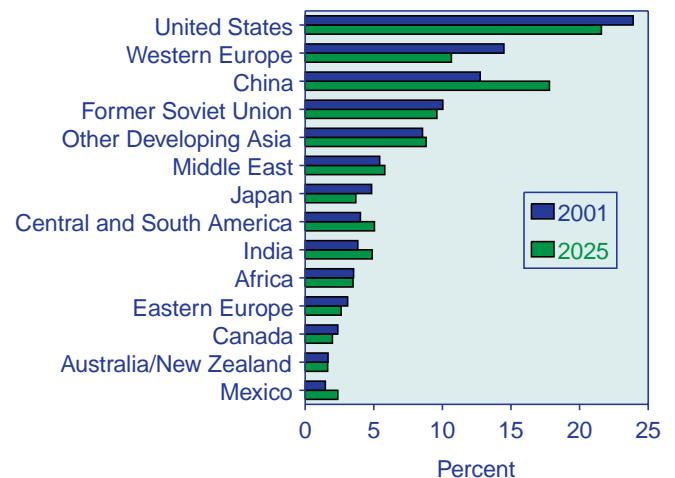
Figure 59. Regional Shares of World Carbon Emissions, 2001 and 2025
