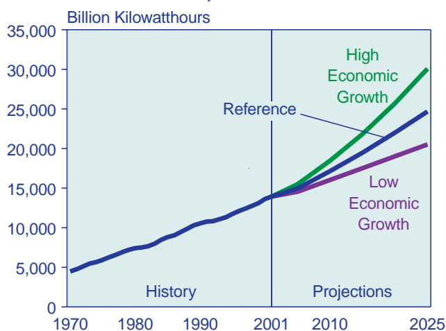
Figure 77. World Net Electricity Consumption in Three Cases, 1970-2025
