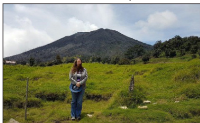
VOLCÁN TURRIALBA, COSTA RICA
