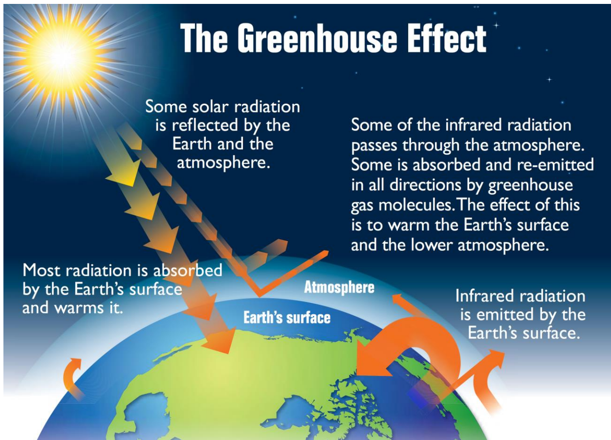
Figure 2.0: The Greenhouse Effect
