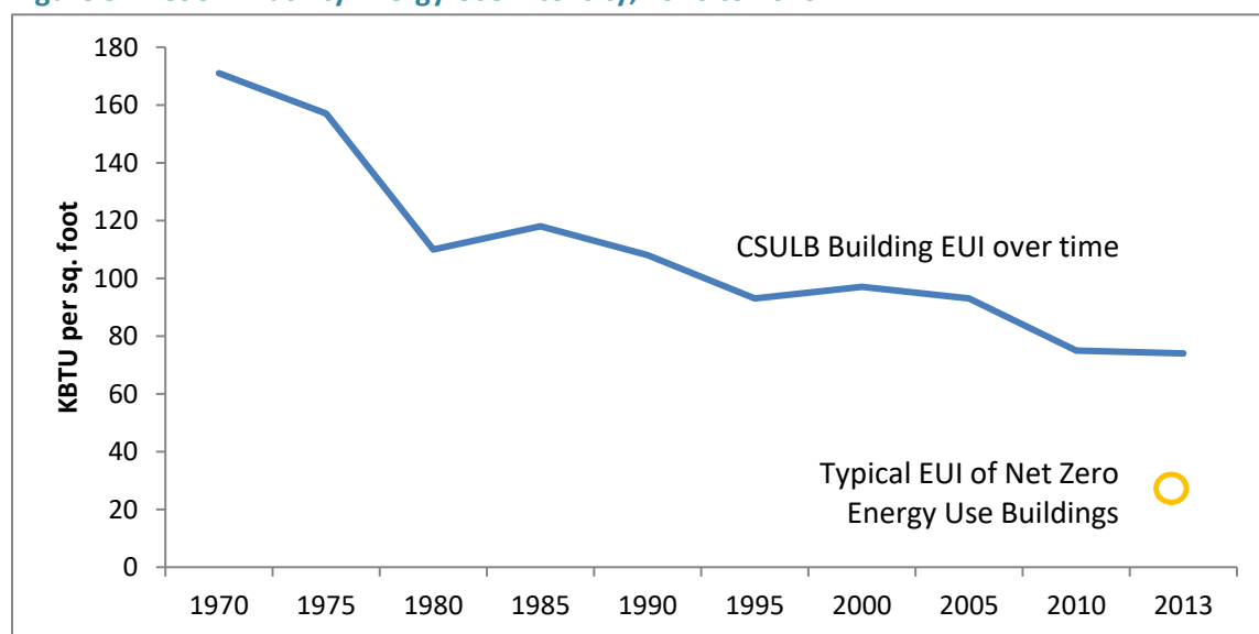
Figure 5.1: CSULB Facility Energy Use Intensity, 1970 to 2013
