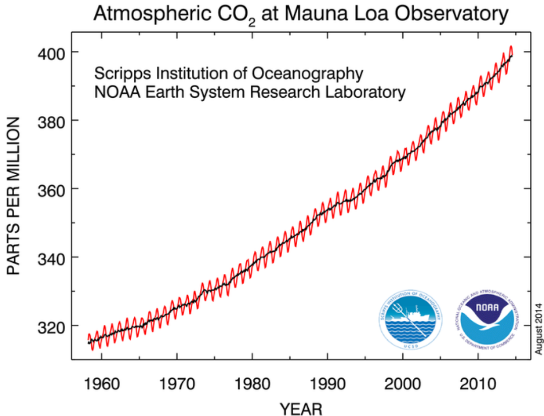
Figure 2.1: Seasonal variation (red line) and annual trend (black line) of atmospheric CO 2 levels
