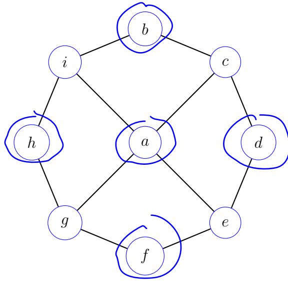
Figure 1: I = \{a, b, d, f, h\} is an independent set for the above graph
