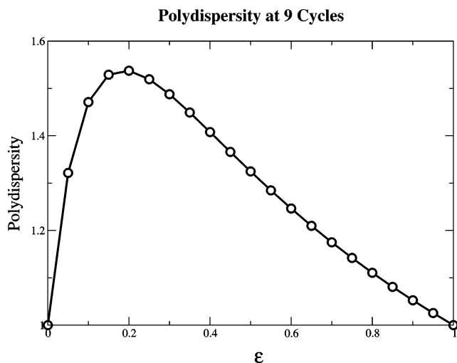
Figure 4. Polydispersity at 9 cycles. The polydispersity M_w/M_N after 9 synthesis cycles is presented at various \epsilon . For small values of \epsilon , the system is nearly monodisperse because relatively few chains have been joined together, and the overall average molecular weight of the chains is nearly 1. As \epsilon \rightarrow 1 , however, the chains grow larger and larger, and all nearly achieve, M_w = 2^9 N .
