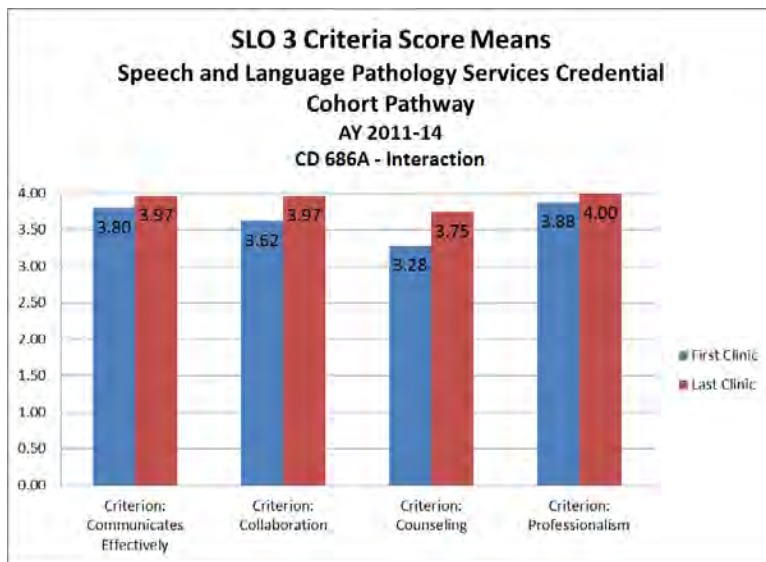
SLO 3 - CD 686A (Cohort)
