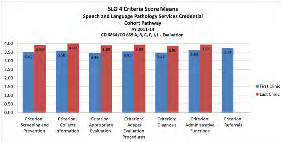
SLO 4 - CD 686A (Cohort)
