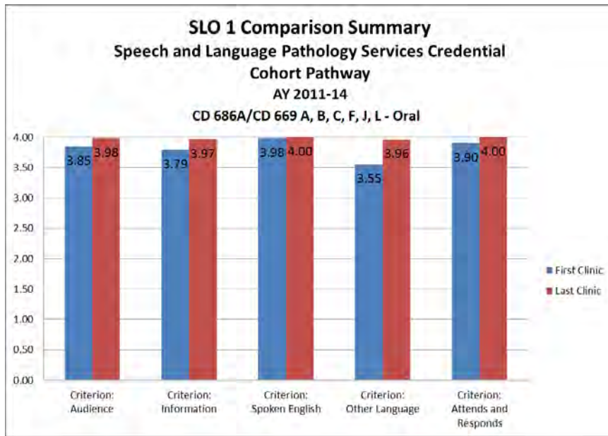
SLO 1 - CD 686A (Cohort)
